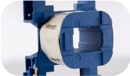
Coil 220V for Contactor D-25
