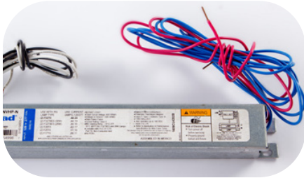
Ballast 2x32W
